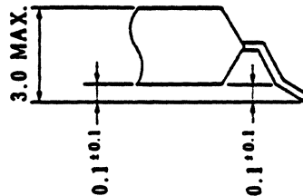
Detail Drawing of Pin Tip Shape
